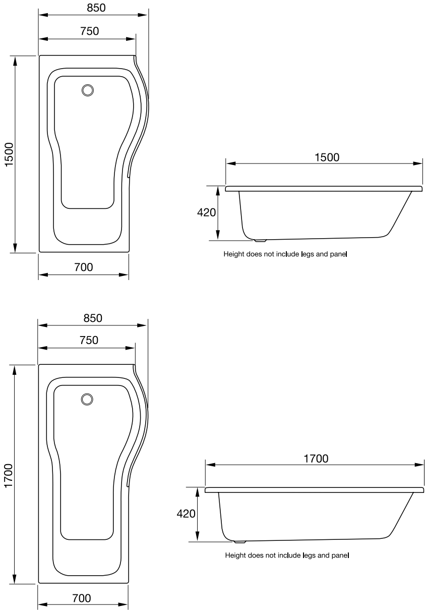
Drawings shows right hand shower bath
