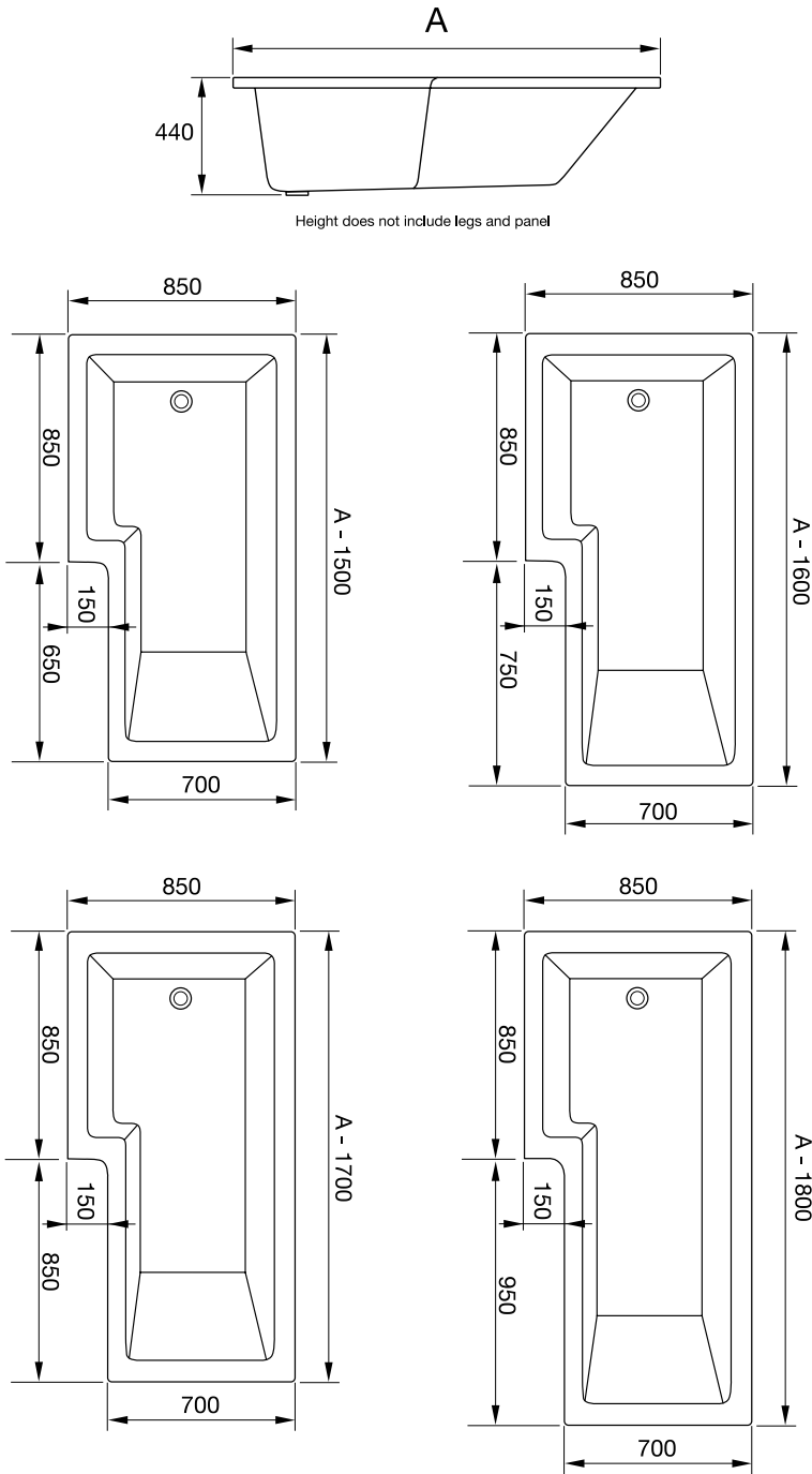
Drawings shows left hand shower bath
